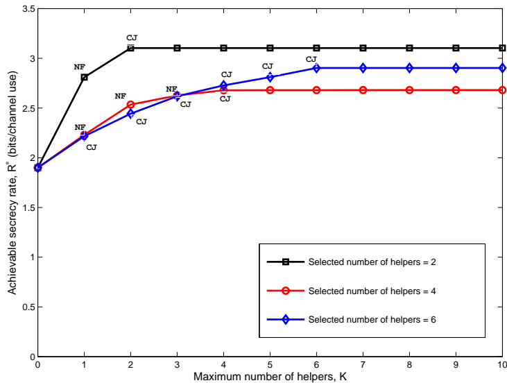
Figure 3.4: The achievable secrecy rate versus the maximum allowed number of helpers, K , for three realizations of relays locations, with N = 50 .
