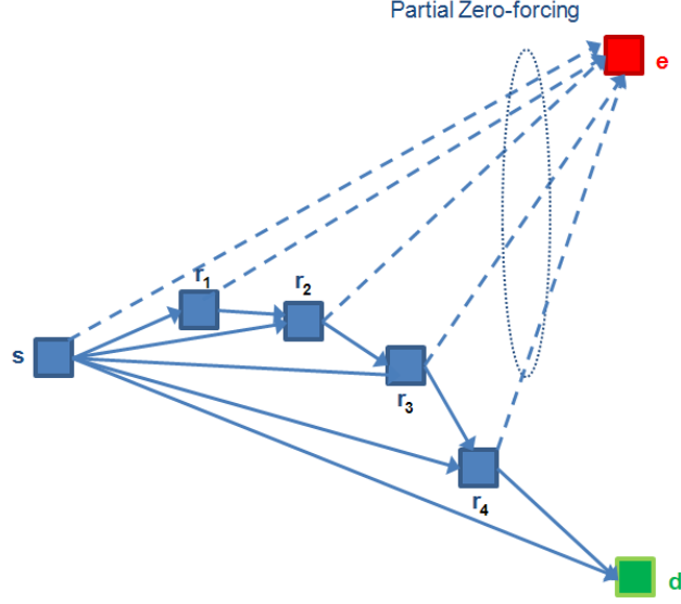
Figure 5.3: Multiple relay multiple hop strategy.
