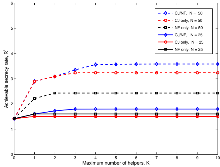
Figure 3.3: The achievable secrecy rate, R^* , versus the maximum allowed number of deaf helpers, K , for three cases: CJ/NF, NF only, and CJ only
