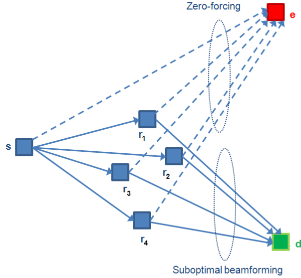
Figure 5.2: Multiple relay single hop strategy.
