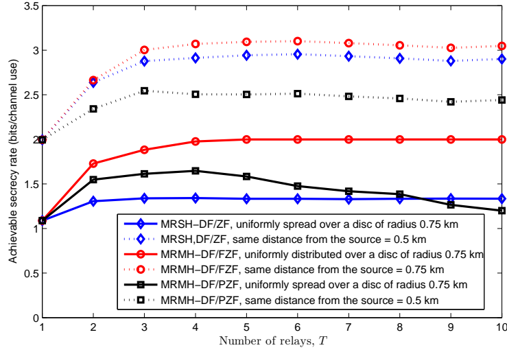
Figure 5.6: The achievable secrecy rate by the MRSH-DF, the MRMH-DF/PZF, and the MRMH-DF/FZF strategies versus the number of relays, T , for two cases.
