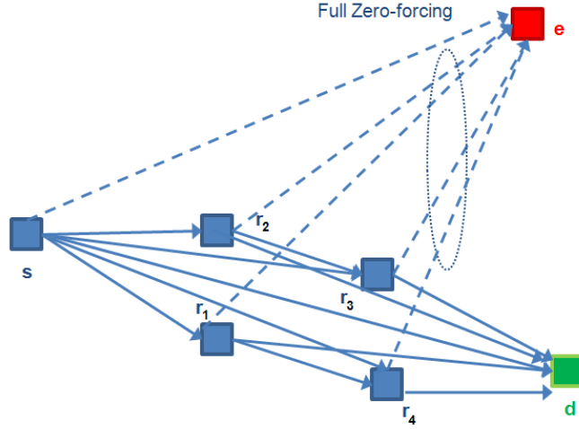
Figure 5.4: Multiple relay multiple hop strategy.
