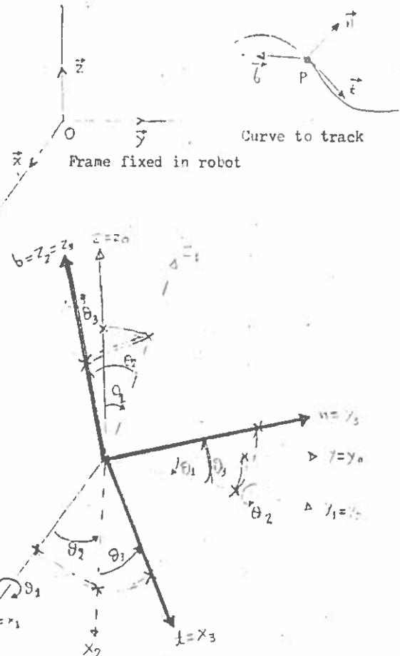
Figure 1. Euler Angles, O Translated to P.
