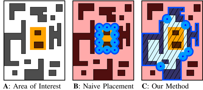
Fig. 1. A: Map of an urban environment projected onto the ground-plane \mathcal{X} \subset \mathbb{R}^2 with obstacles \mathcal{X}_{obs} (dark) and a user defined region of interest \mathcal{X}_{int} (orange) for which access must be monitored or guarded. B: Many agents (dark dots) may be required to cover the boundary of \mathcal{X}_{int} with sensors (blue discs). C: Our method uses fewer agents by placing agents at the bottlenecks created by obstacles. This creates a safe region of isolation \mathcal{X}_{iso} (shaded blue area) containing the region of interest, \mathcal{X}_{int} \subset \mathcal{X}_{iso} .
