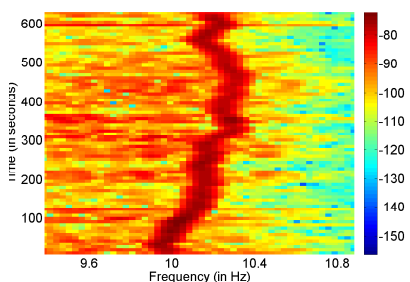
(b) ENF signal from the video track
