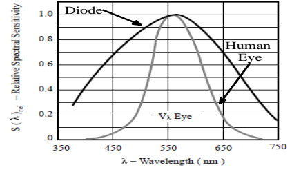
Figure 1: Spectral sensitivity of BPW21 photo diode (From: Vishay Semiconductor Web Catalog).
