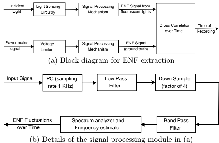
Figure 4: Block diagram for estimating the time of recording of sensor signal.
