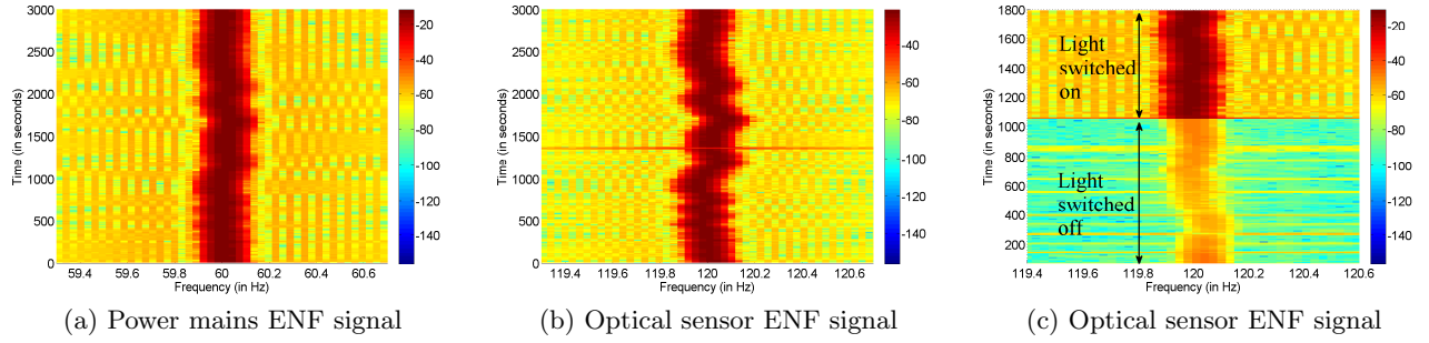
Figure 5: (a),(b) ENF fluctuations of signals captured in Experiment 1; (c) ENF for sensor signal in Experiment 2, including a weak signal for first 17 minutes from the ambient light, when the main light is switched off.
