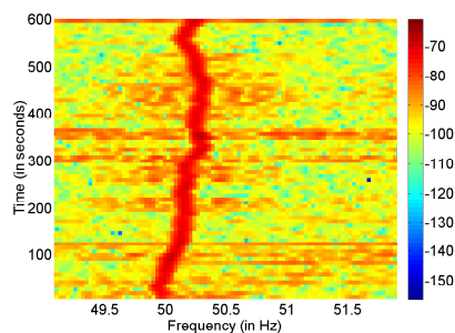
(a) ENF signal from the audio track
