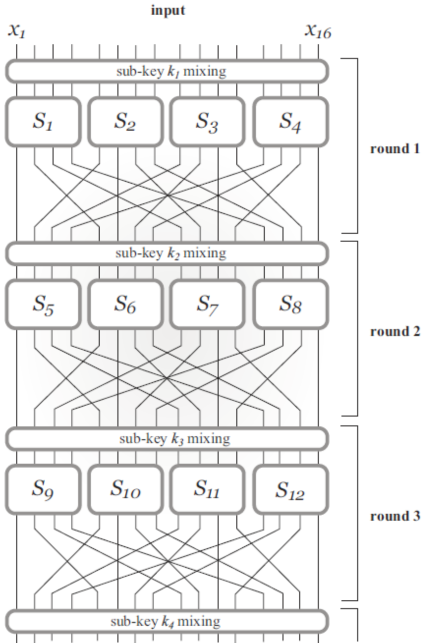
FIGURE 6.2: A substitution-permutation network.
