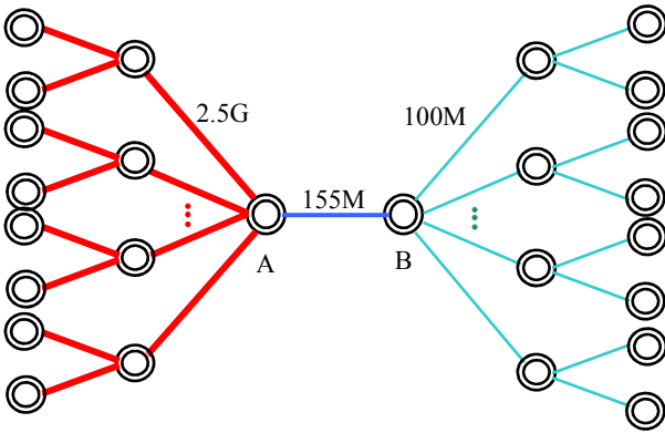
Fig. 10. Sample Network with EF PHBs for Voice and Video Services
