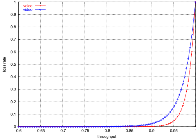
Fig. 11. QoS Behaviors for Voice and Video Services
