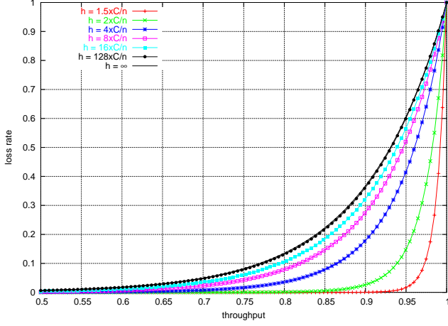
Fig. 6. Relation between Loss Rate and Throughput for Different Link Speeds
