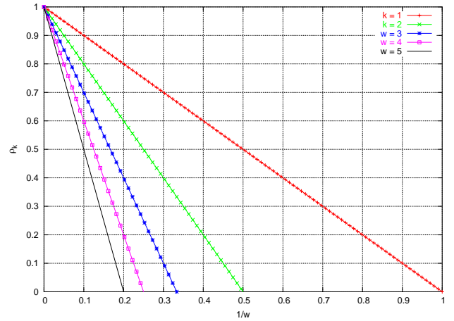
Fig. 5. Change of k -th QoS Region with Burst Size
