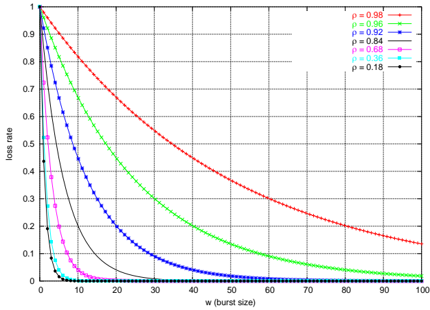
Fig. 3. Relations between Loss Rate and Burst Size for Different Throughputs
