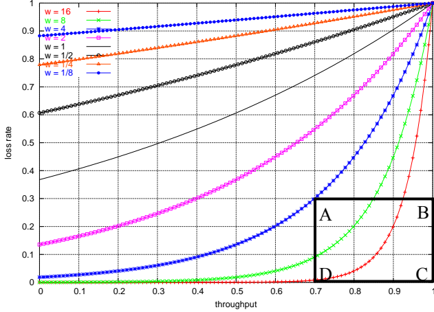
Fig. 2. Relations between Loss Rate and Throughput for Different Burst Sizes
