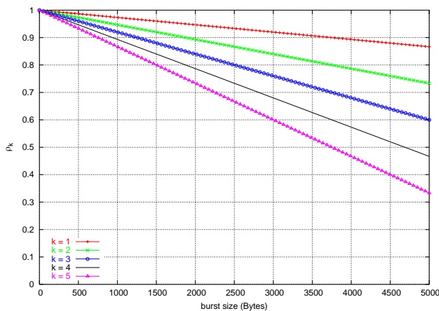
Fig. 13. Change of QoS Regions with Burst Size for Video Service
