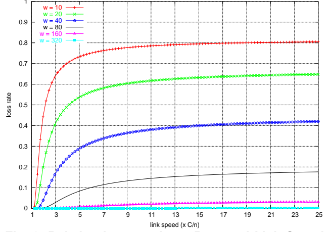
Fig. 8. Relation between Loss Rate and Link Speed for Different Burst Sizes
