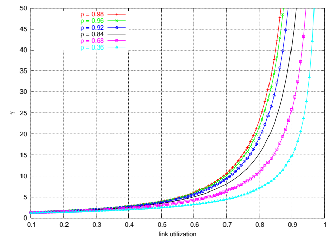
Fig. 9. Change of Shaping Factor with Link Speed for Different Network Utilities
