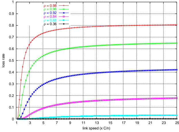
Fig. 7. Relation between Loss Rate and Link Speed for Different Throughputs
