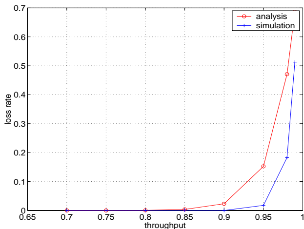
Fig. 15. Comparisons of the Analytical and the Simulated QoS Behaviors for the Video Service
