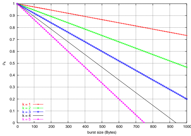
Fig. 12. Change of QoS Regions with Burst Size for Voice Service
