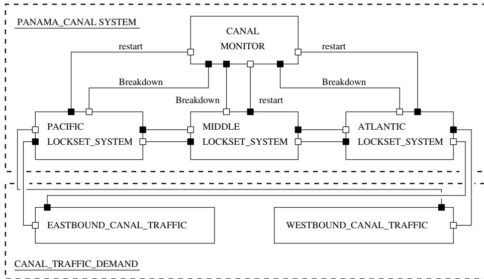
Figure 15. Process architecture for full canal model.
