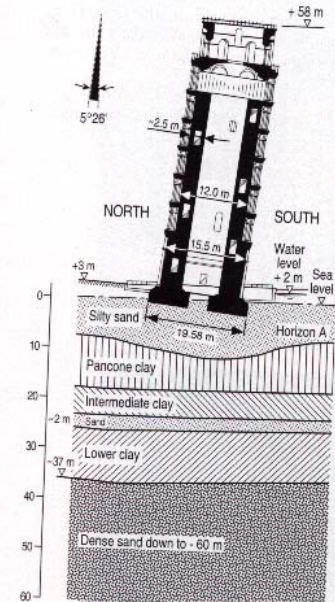
Fig. 2: Soil profile
