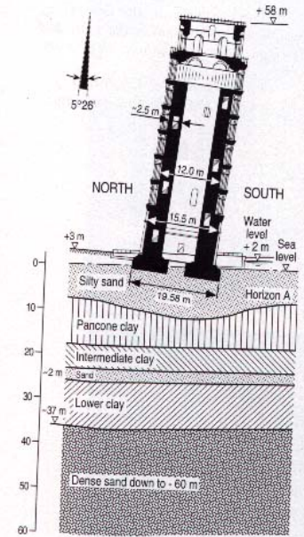
Fig. 2: Soil profile
