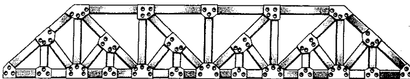
Baltimore or subdivided Pratt (e)
