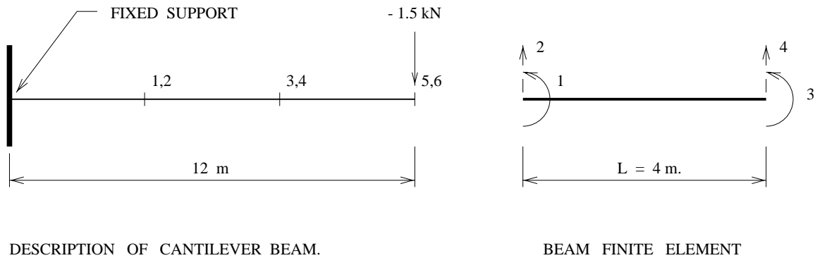
DESCRIPTION OF CANTILEVER BEAM.
