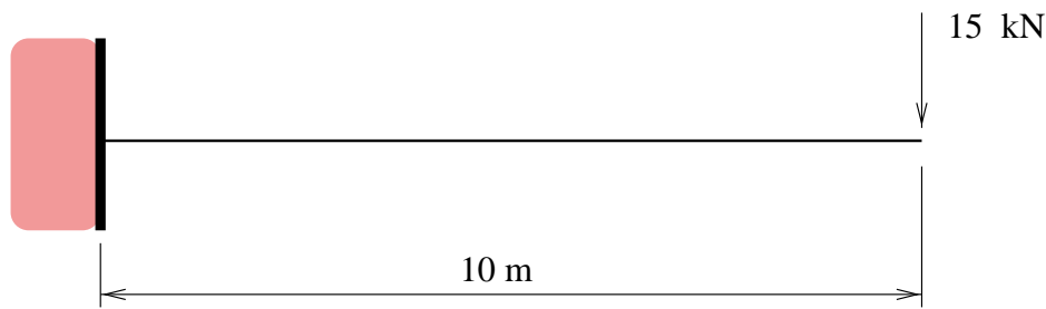
(a) : Cantilever Beam and Point End load
