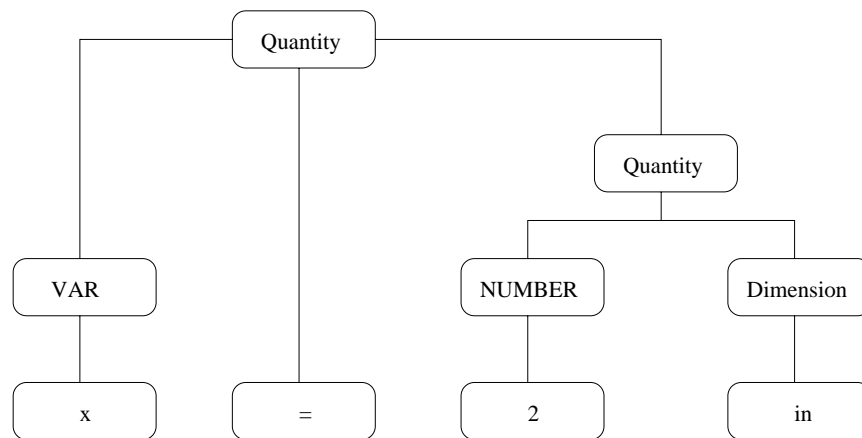
FIG. 10. : Parse tree for x = 2 in
