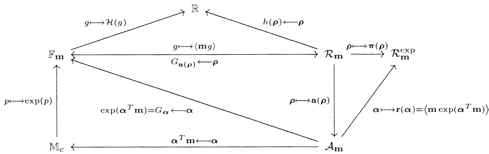
FIG. 1. A commutative diagram summarizing mappings and relationships between important sets.
